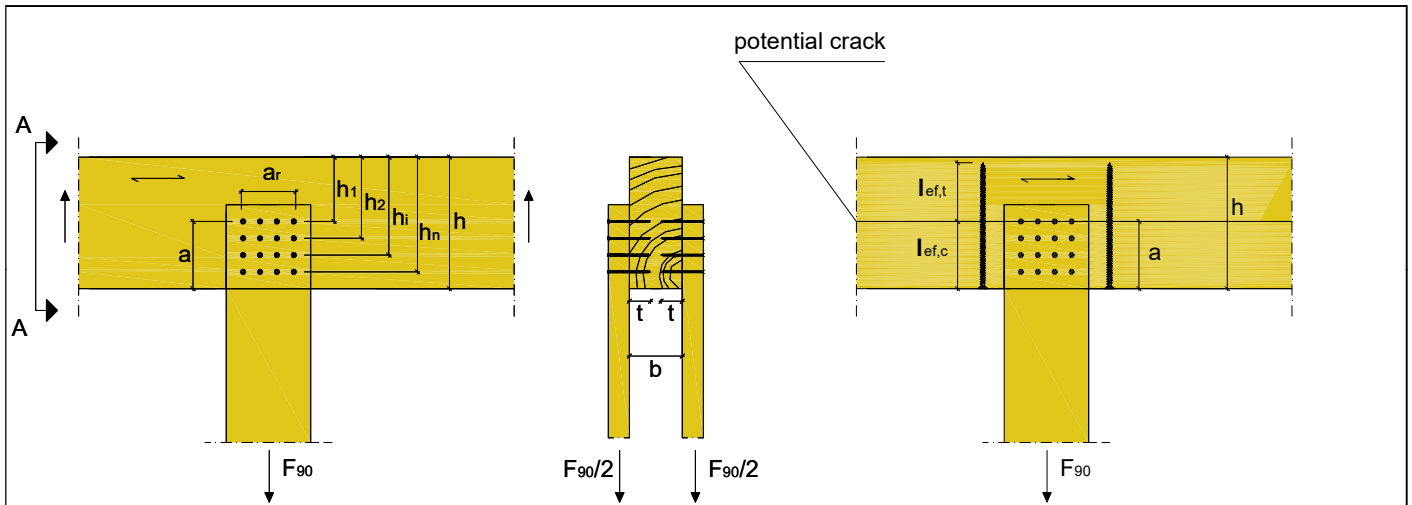
Figure A.4.1 Example for tensile reinforcement of a connection force perpendicular to the grain
