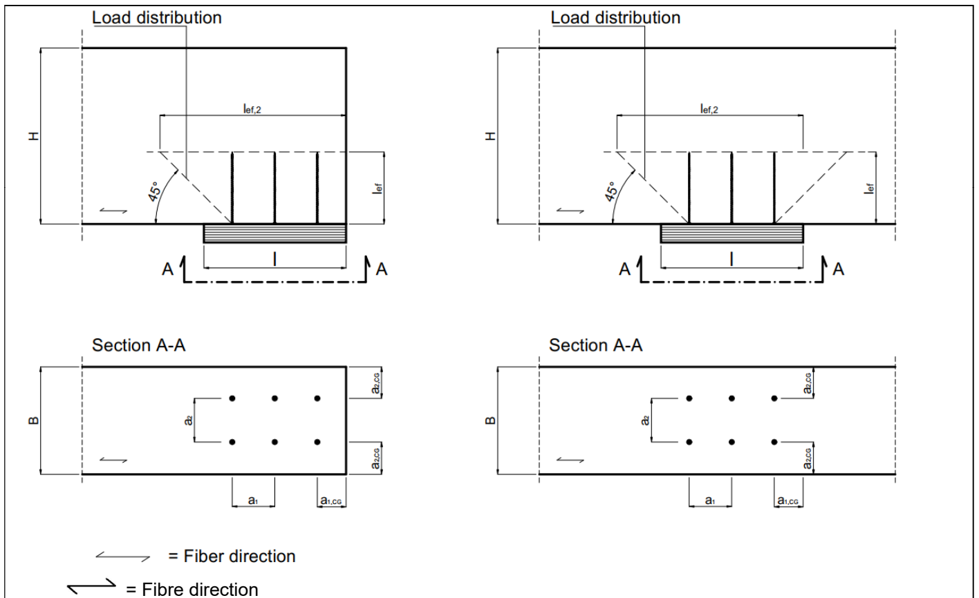
Figure A.3.1 Reinforced end support (left) and reinforced intermediate support (right)
