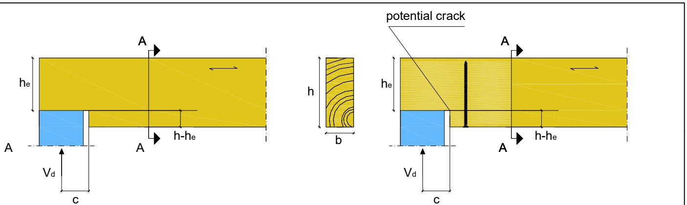
Figure A.4.2 Example for tensile reinforcement of a notched beam support
