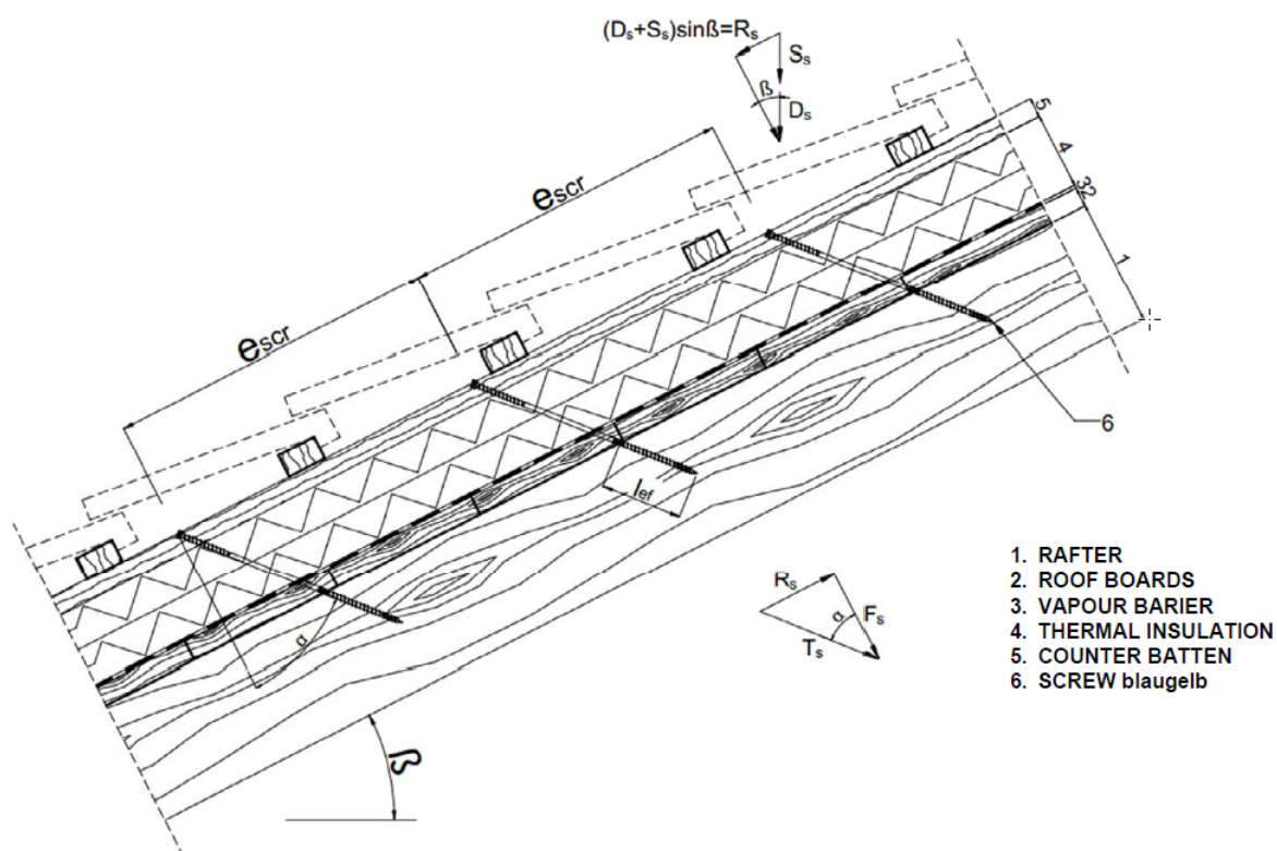
Figure A.6.3 Point loads F_s perpendicular to the counter battens, load application in the area of the screw heads
