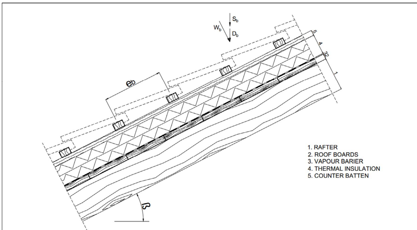
Figure A.6.2 Point loads F_b perpendicular to the counter battens
